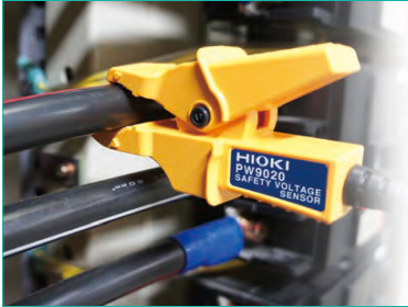
Freely clip either horizontally or vertically
