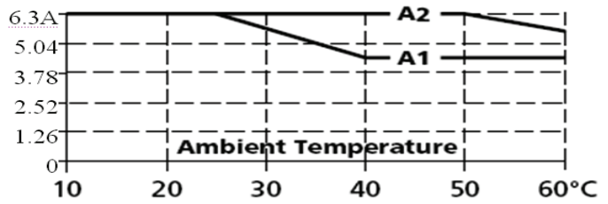
Output Current
