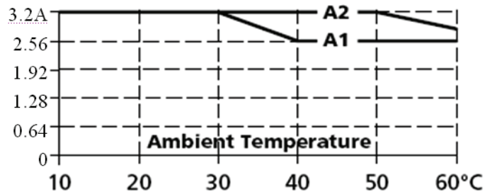
Output Current
