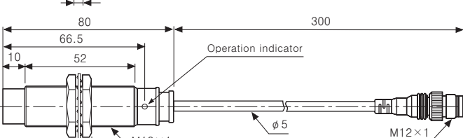
●PRWL18-8A□
