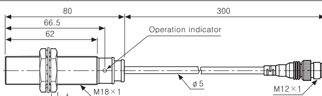
●PRWL18-5A□
