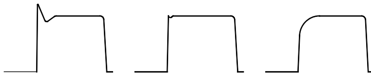
Over-compensated, correct, and under-compensated waveforms
