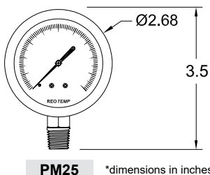
PM25 *dimensions in inches
