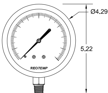
PM40 *dimensions in inches
