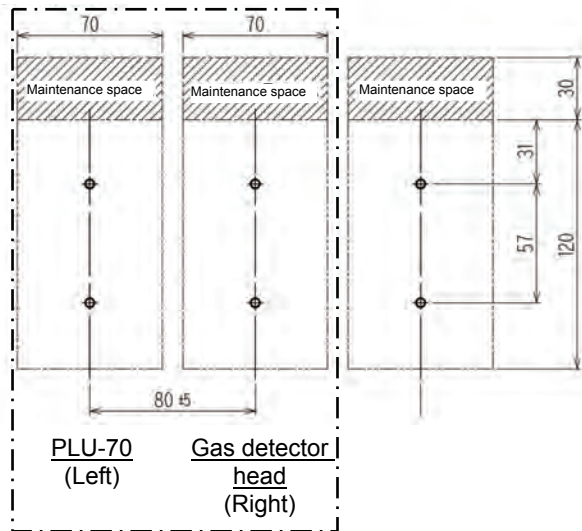
When installing by using 2 screws
