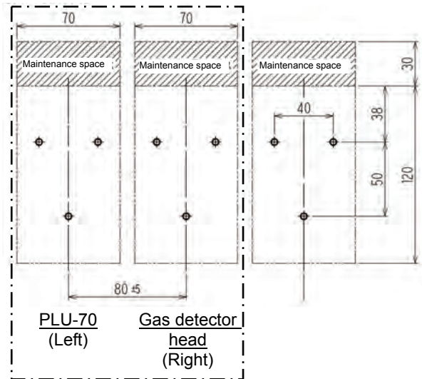
When installing by using 3 screws
