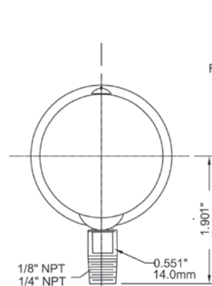
2" Bottom Connection
