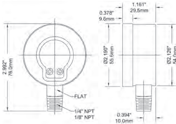
2.5" Bottom Connection
