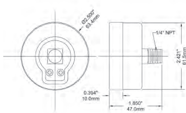
2.5" Back Connection
