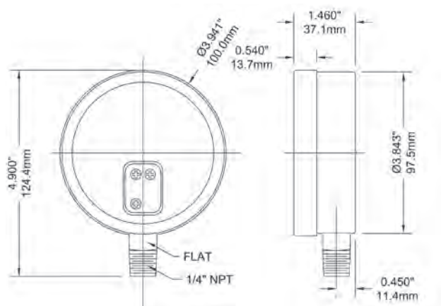
4" Bottom Connection
