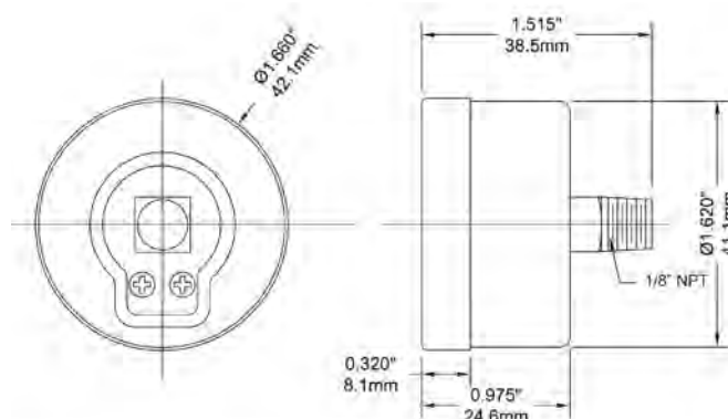
1.5" Back Connection
