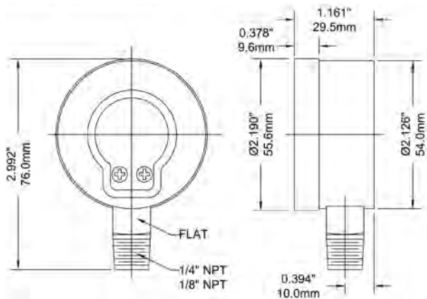
2.5" Bottom Connection
