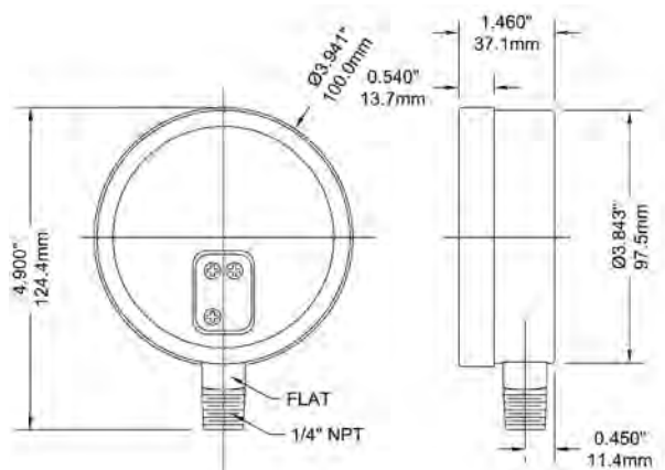
4" Bottom Connection
