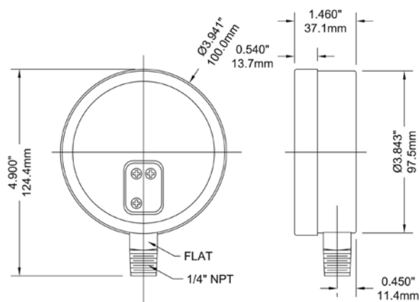
4" Bottom Connection
