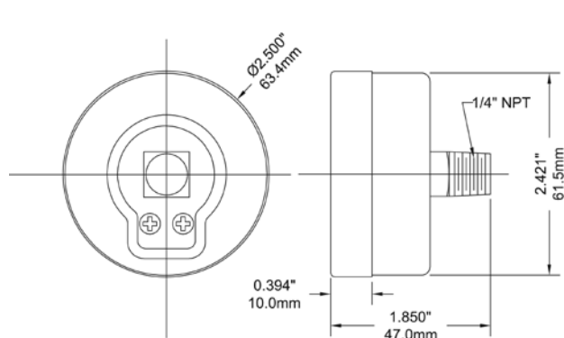
2.5" Back Connection
