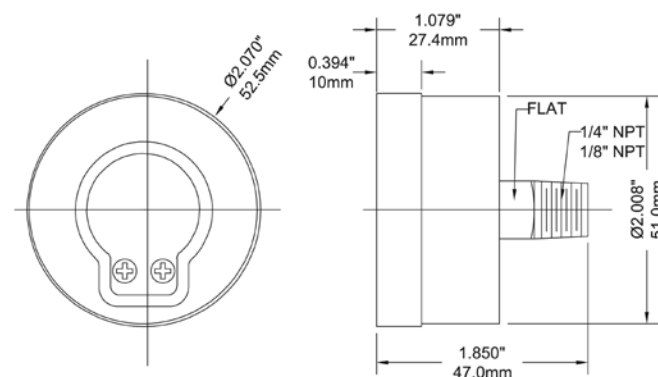
2" Back Connection
