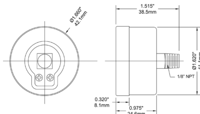
1.5" Back Connection
