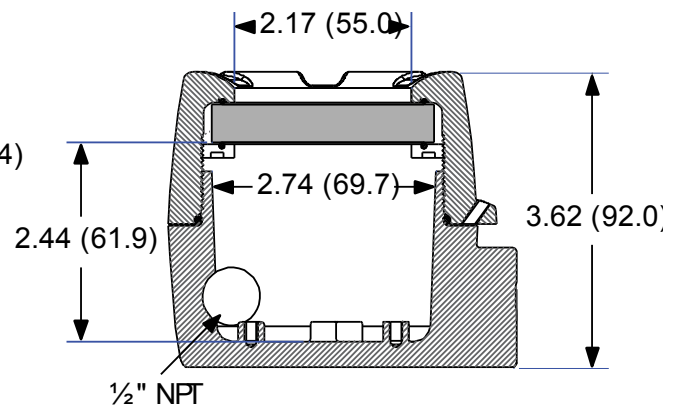
Figure 4. Enclosure Dimensions – Side Cross Section View
