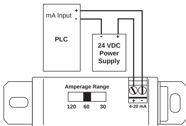
Figure 5: PDA6420 being powered by external 24 VDC power supply such as Precision Digital model PDA1024-01.
