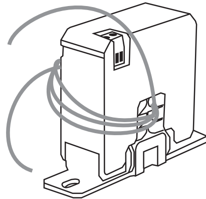
Figure 2: PDA6420 Current Transducer Shown with Four Turns
