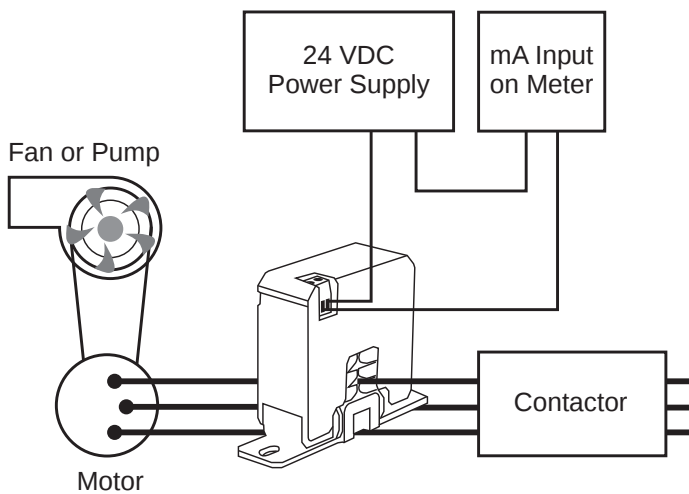
Figure 1: Measuring Current Using PDA6420 Current Transducer
