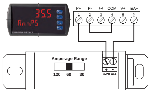
Figure 6: PDA6420 being powered by the Precision Digital PD6000. PD6000 is displaying the current being measured by the PDA6420.
