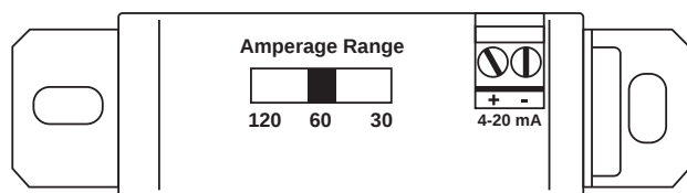
Figure 4: Current Setting Switch
