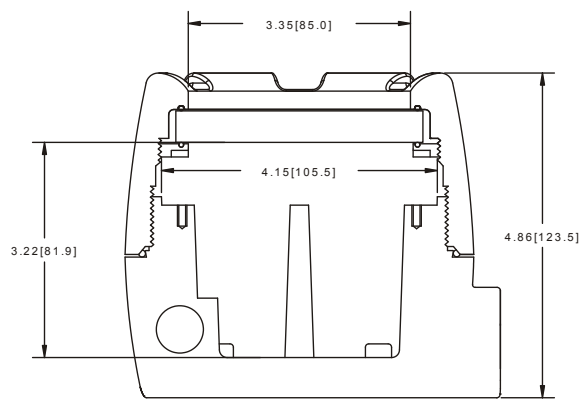
Figure 17. Enclosure Dimensions – Side View
