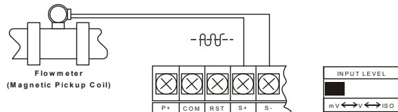
Figure 4. Self-Powered Magnetic Pickup Coil Flowmeter (Coil)
