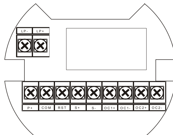
Figure 1. Connector Board
