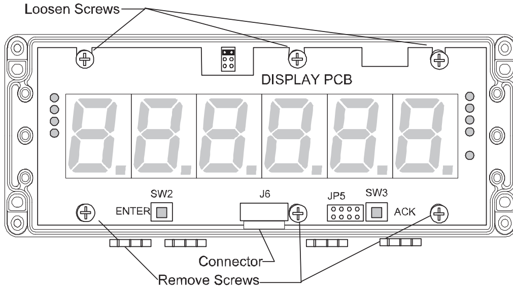
Figure 32. Removing the Display Board
