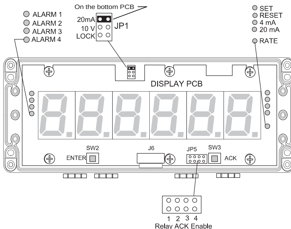
Figure 14. Jumper Arrays and Status LED Identification
