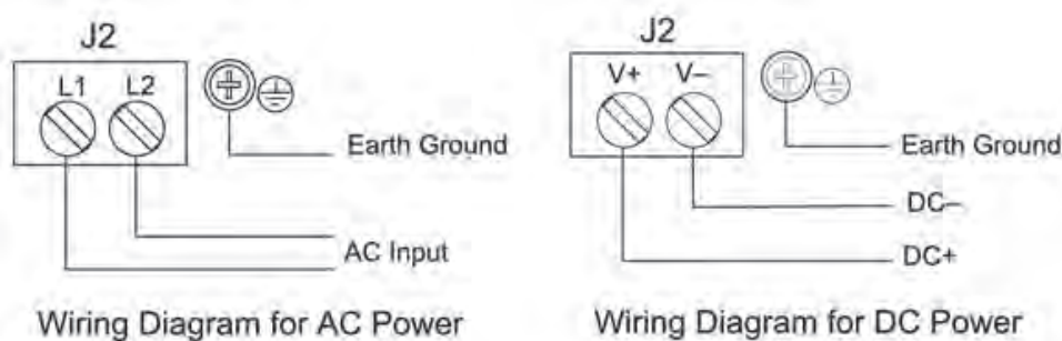
Figure 5. Input Power Connections
