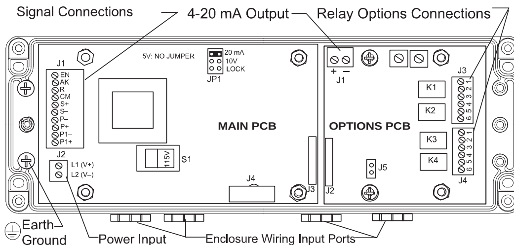
Figure 3. Connections and Jumper Diagram
