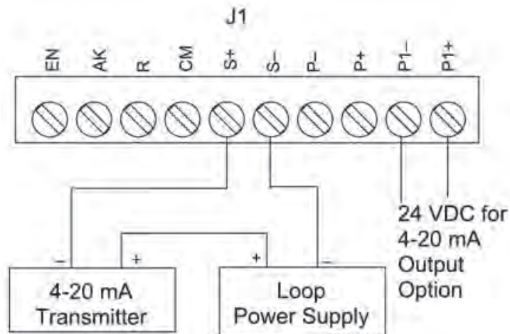
Figure 7. Two-Wire Transmitter Powered by External Supply
