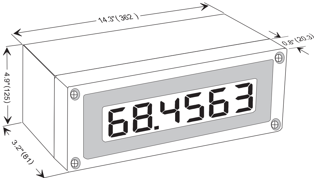
Figure 28. Overall Dimensions
