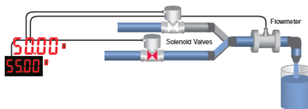
Multi-Stage Batch Control
