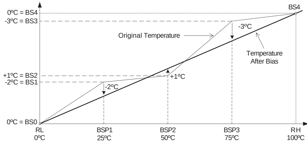
Fig 1: Temperature Bias
