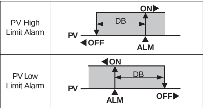
Fig 3: Alarm Operation
