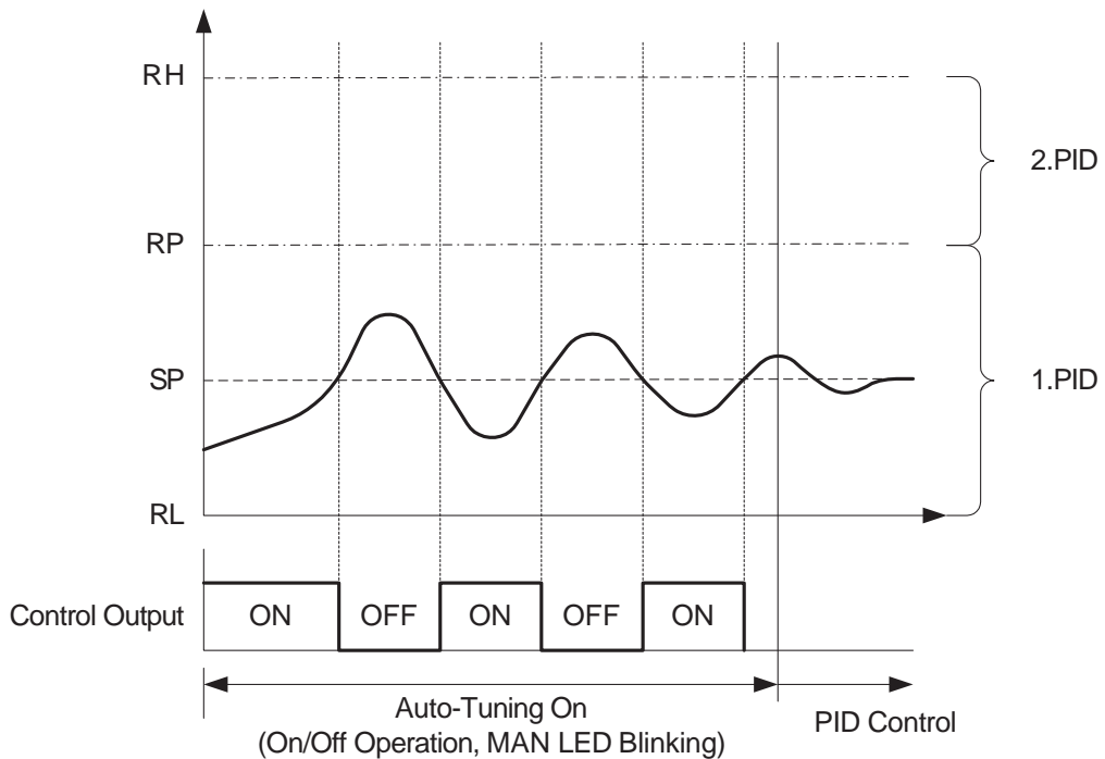
Fig 9: Auto-Tuning
