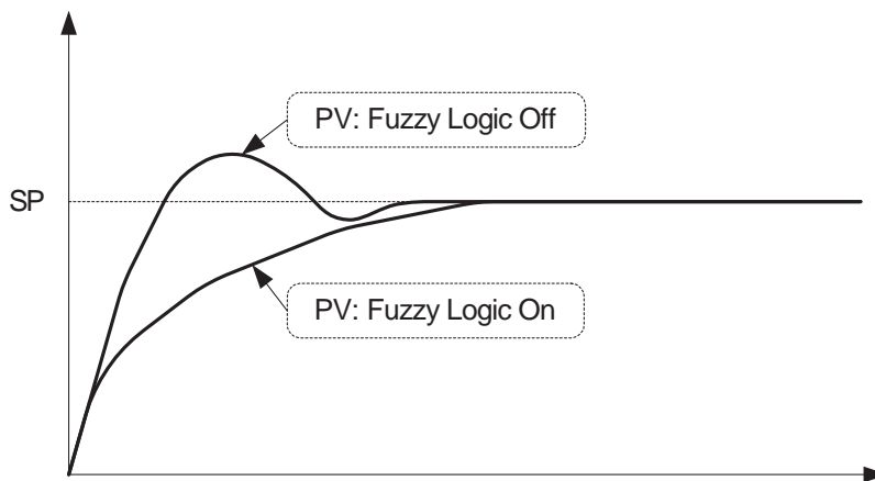
Fig 5: Overshoot Suppression with Fuzzy Logic
