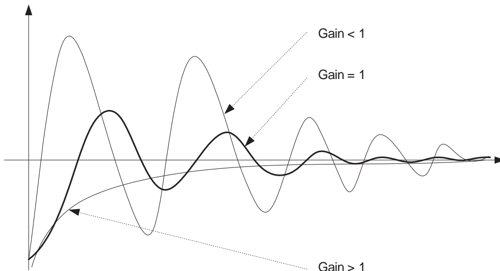
Fig 10: Auto-Tuning Gain
