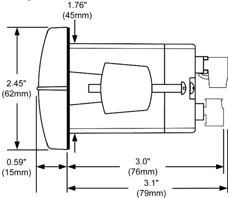
Figure 3. Case Dimensions – Side View
