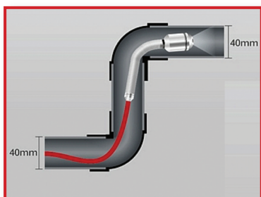
Eight super-bright white LEDs give the DPS16/ P16PIP probe 640 x 480 pixel (VGA) resolution
