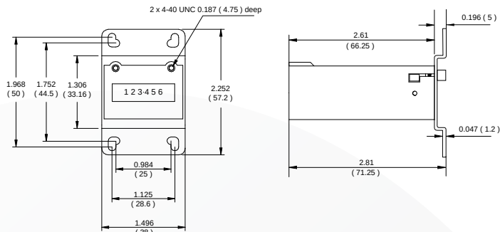
V - V-Base Mount / RV- Combo Front / V-Base Mount
