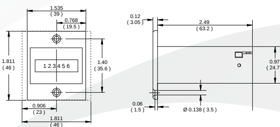
P - Panel Mount (Flange) 1.81 x 1.81(46 x 46)
