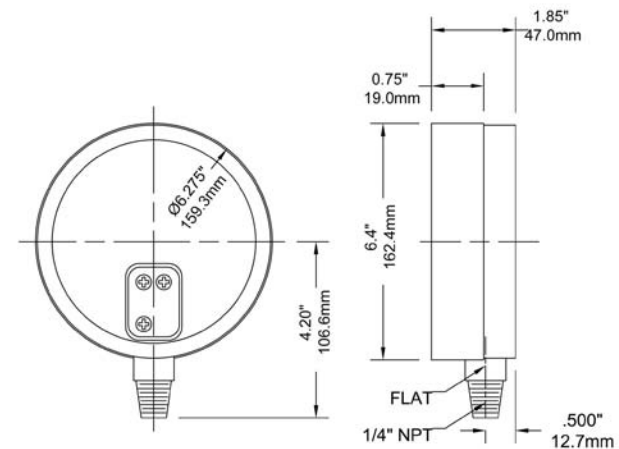
6" Bottom Connection
