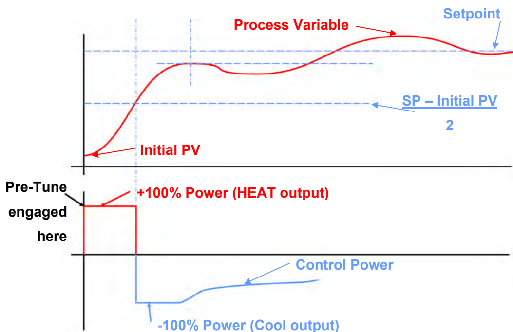
Figure 44. Pre-Tune Operation
