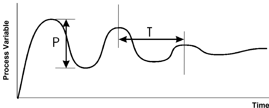
Figure 39. Manual Tuning
