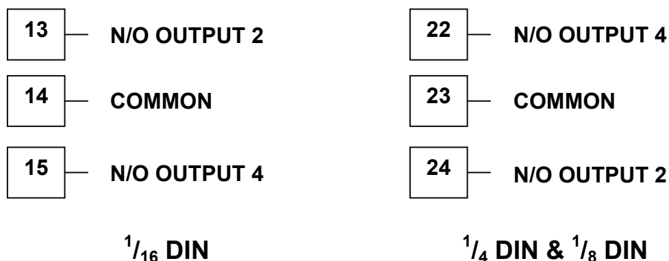
Figure 25. Option Slot 2 - Dual Relay Module
