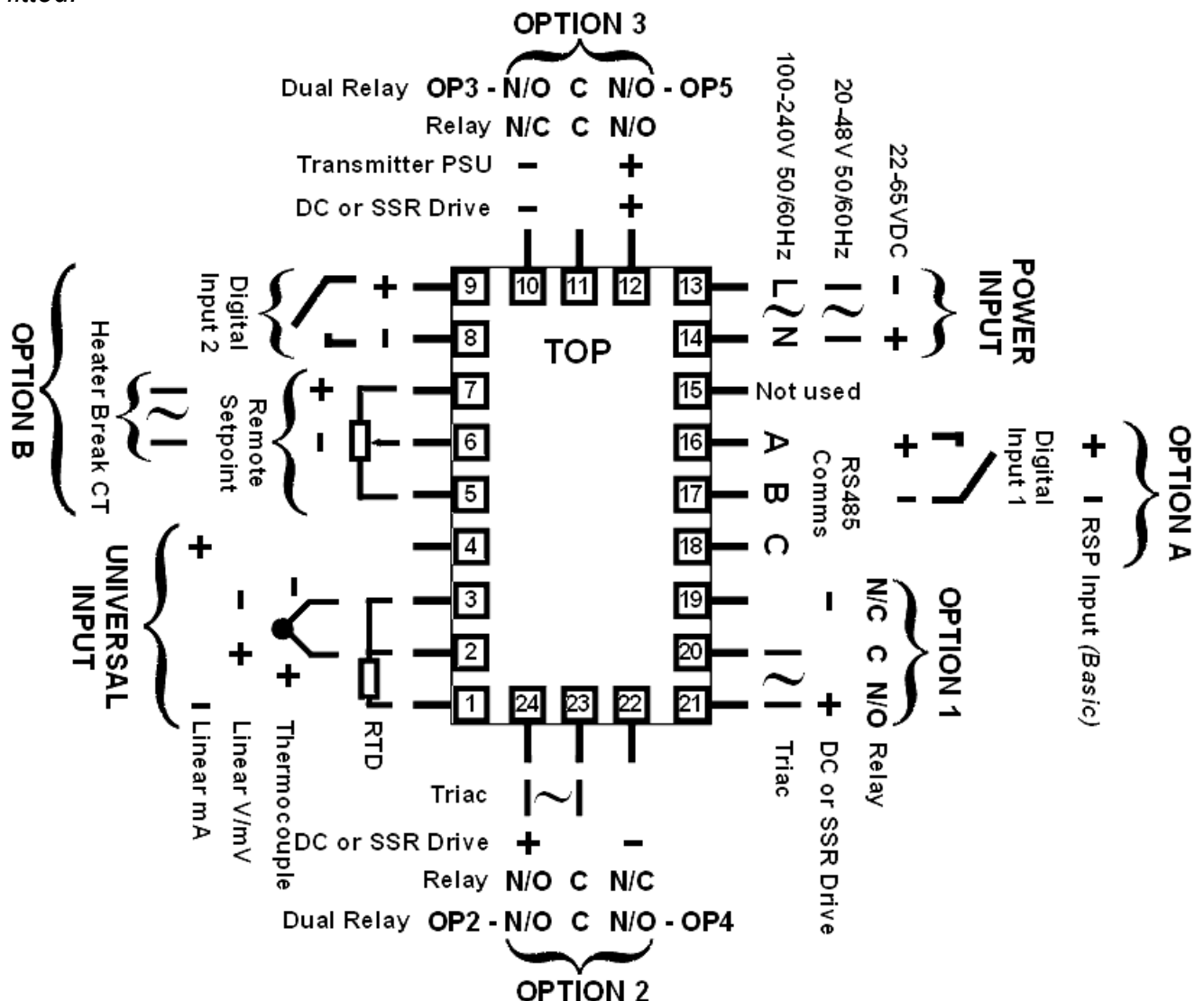
Figure 12. Rear terminals ( \frac{1}{4} -DIN & \frac{1}{8} -DIN Instruments)
