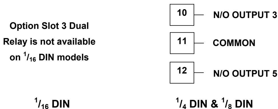
Figure 30. Option Slot 3 - Dual Relay Module
