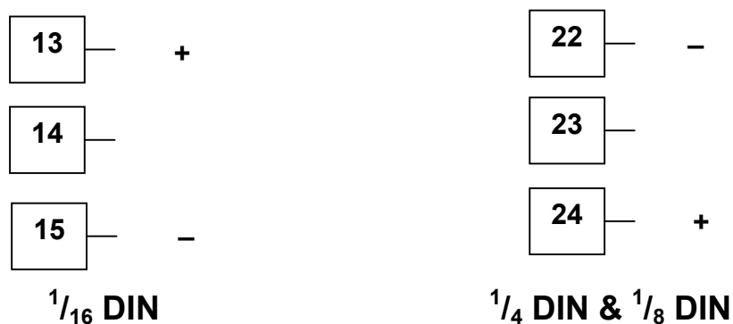
Figure 26. Option Slot 2 - Linear Voltage & mADC module
