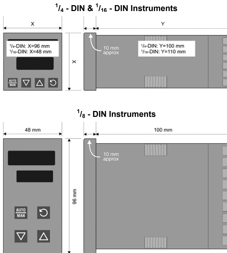
Figure 1. Main dimensions
