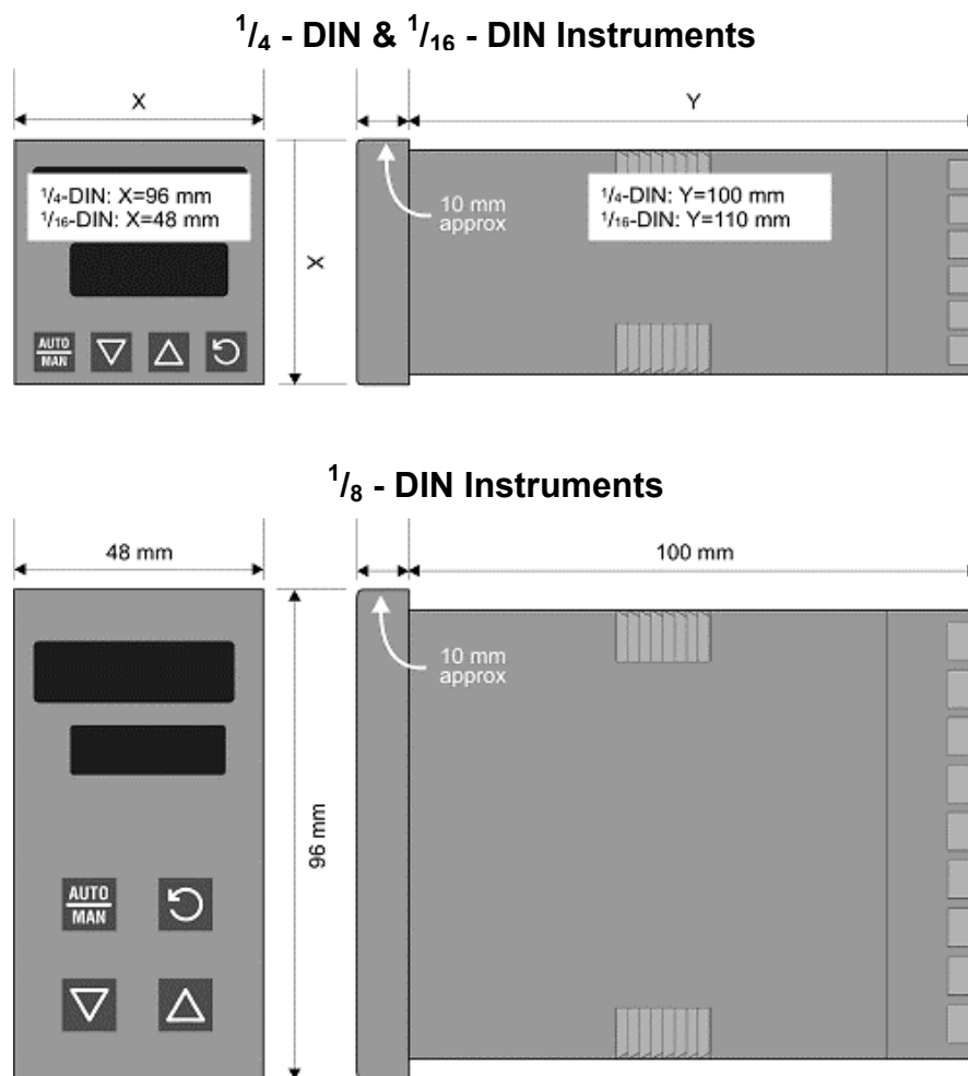
Figure 1. Main dimensions
