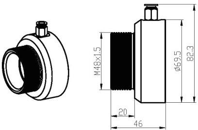
Air Purge Collar (Option)
