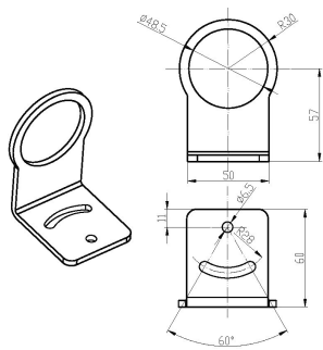
Fixed Bracket
