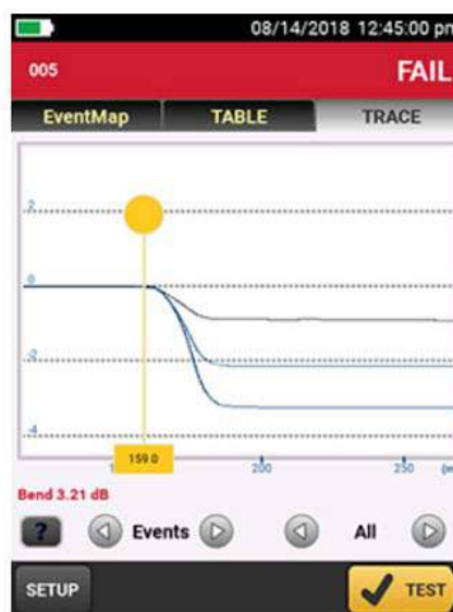
Bend as seen on an OTDR trace
