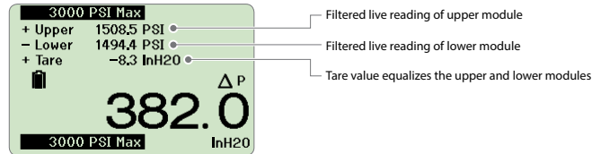
Differential Mode
