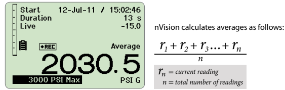
Averaging Mode
