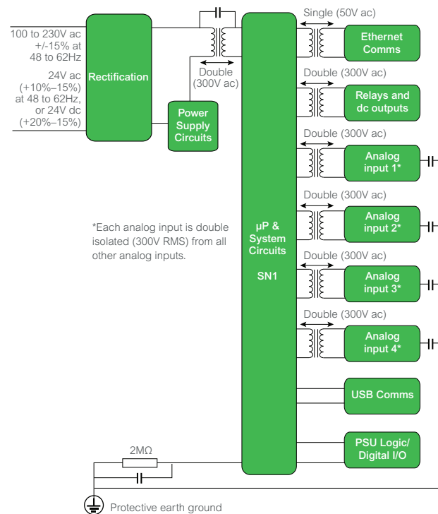
Isolation details
