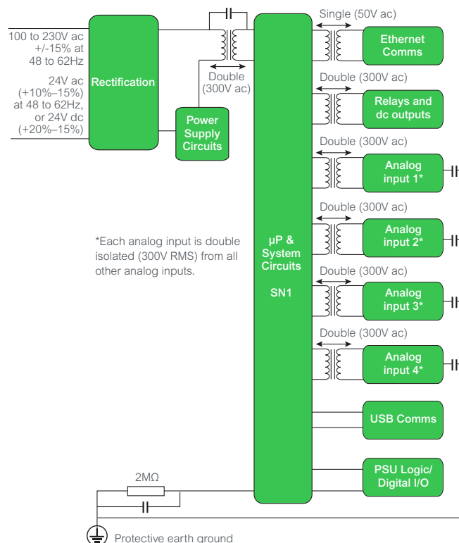
Isolation details
