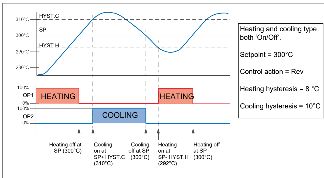
Figure 217 Deadband OFF
