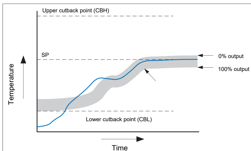
Figure 203 Cutback operation
