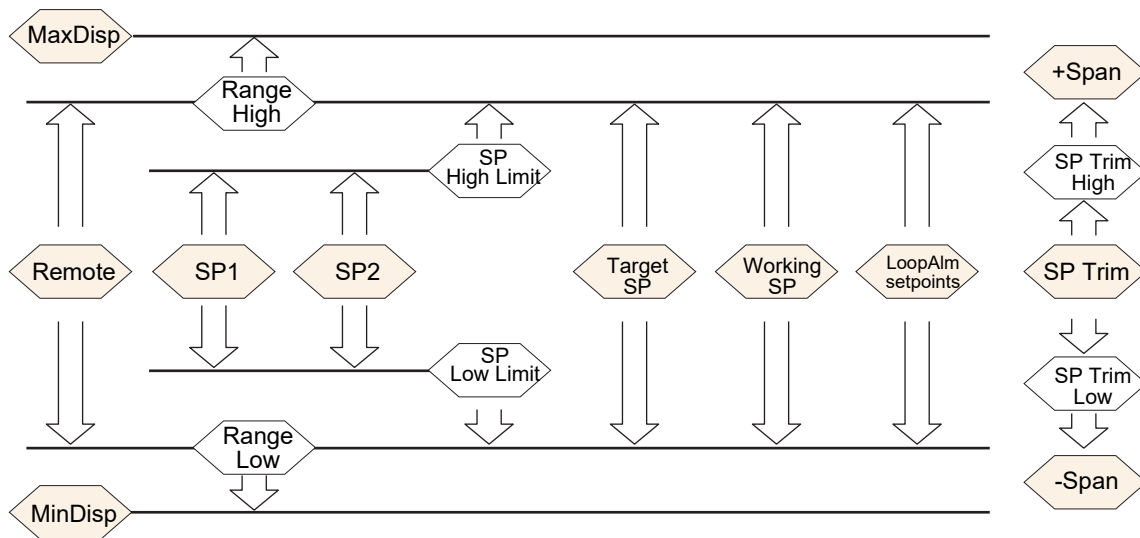
Figure 214 Setpoint Limits
