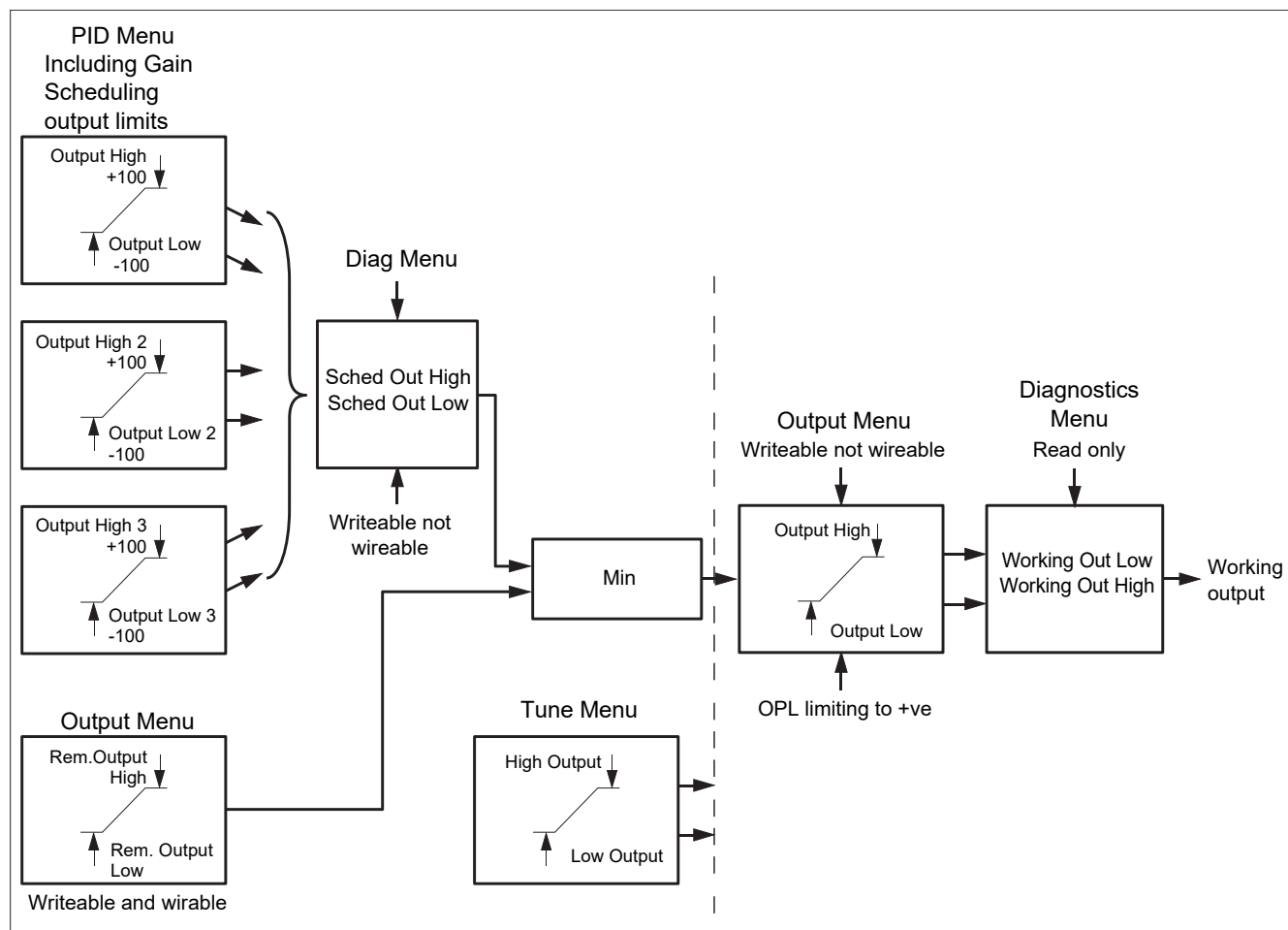
Figure 215 Output Limits
