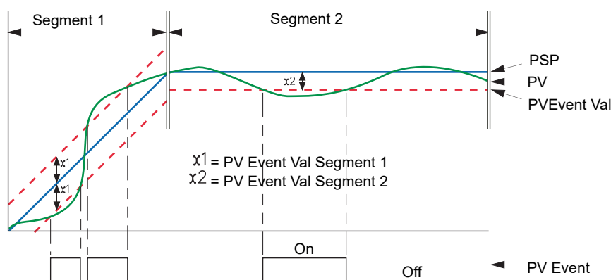
Figure 34 PV Events
