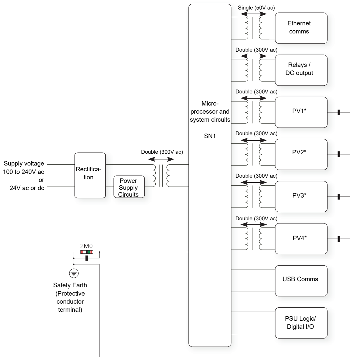
Figure 224 Isolation diagram
