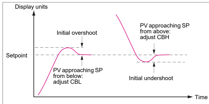
Figure 212 Manual Cutback setting
