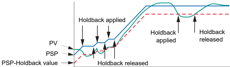
Figure 32 Holdback
