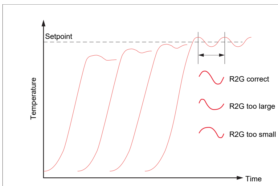
Figure 211 Relative Cool Gain
