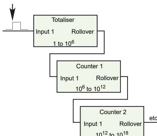
Figure 101 Cascading counters
