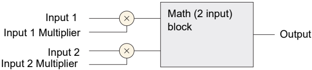
Figure 149 Block schematic
