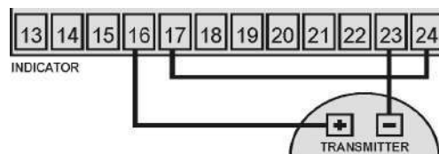
Fig. 9 – Two-wire transmitter with internal power supply
