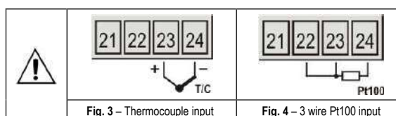
Fig. 3 – Thermocouple input
