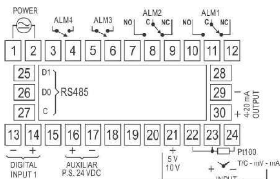
Fig. 1 – Back panel terminals
