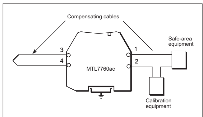
Figure 21: Calibration with thermocouple barrier circuit
