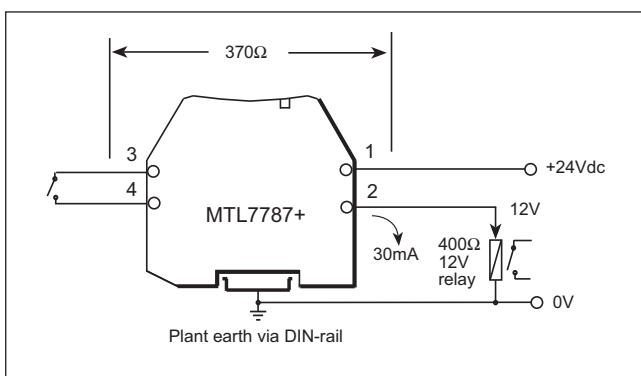
Figure 20: Circuit diagram for testing an MTL7787+ barrier
