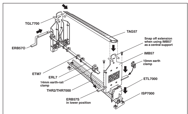
Figure 12: Tagging strip assembly
