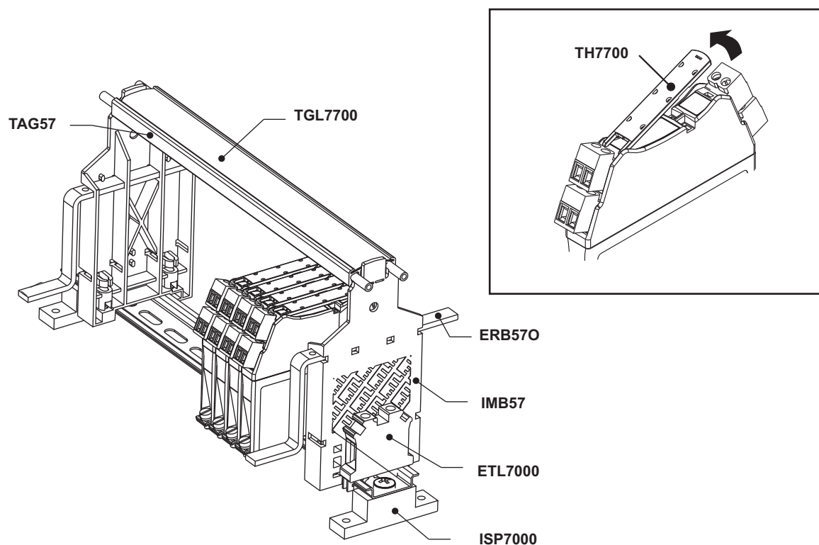
Figure 2: MTL7700 Series mounting and tagging accessories
