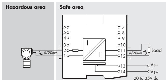
Figure 6.37: MTL5041 wiring diagram and connections
