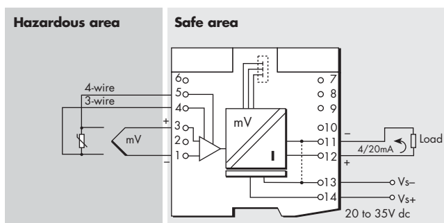
Figure 6.61: MTL5073/74 wiring diagram
