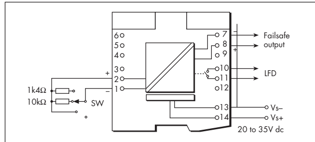
Figure 6.72: Test circuit for MTL5113P
