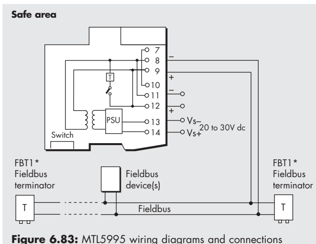
Figure 6.83: MTL5995 wiring diagrams and connections
