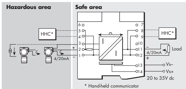
Figure 6.38: MTL5042 wiring diagram and connections
