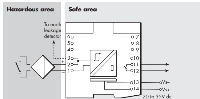
Figure 6.1: MTL5011 wiring diagram and connections
