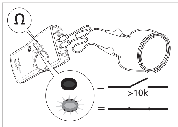
Figure 4. Continuity Test
