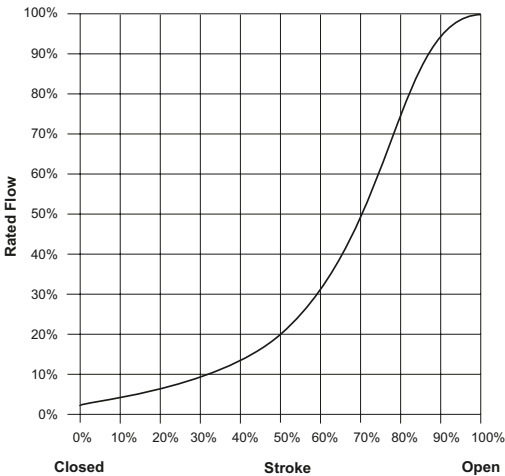
Figure 1. Typical Modified Equal Percentage Flow Characteristics
