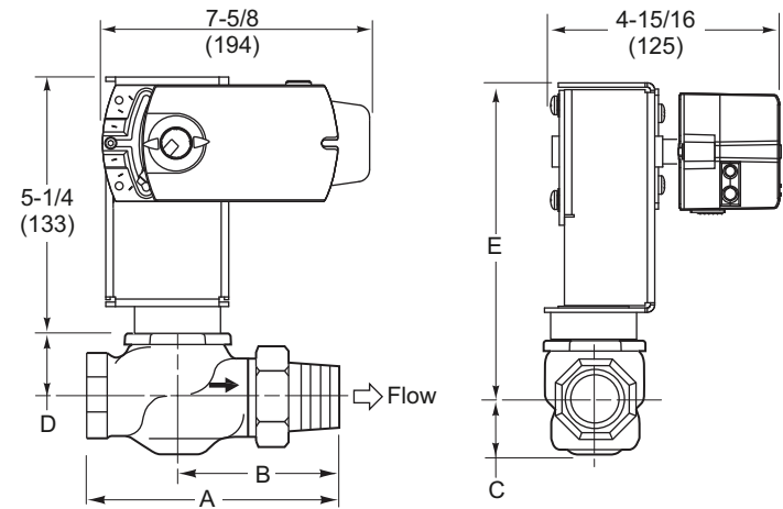
Figure-10 Mx41-6043 or Mx41-6083 with 2-Way Union Straightway Globe Valve with AV-611 Linkage.
