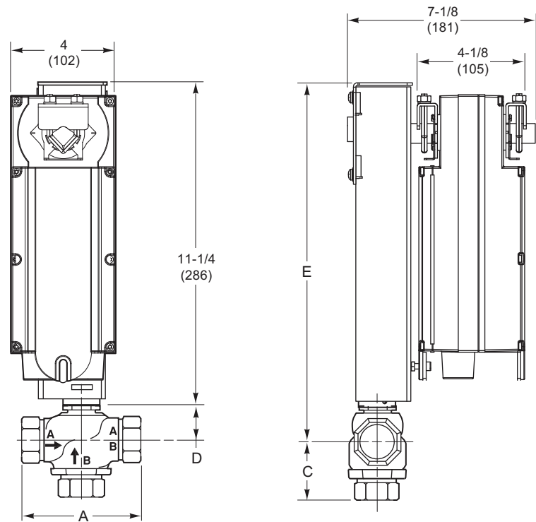
Figure-35 Mx40-717x with 1/2" or 2" 3-Way Globe Valve With AV-602 Linkage.
