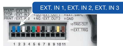
Control terminals
