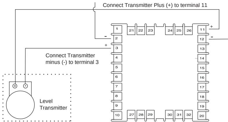
Figure 3 - Transmitter Wiring
