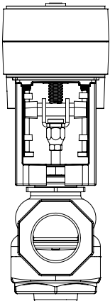
End View Side View MG350V Installed on a VB-7000 Globe Valve
