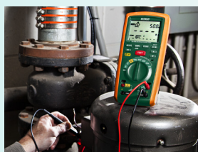
Insulation test on pump motor
