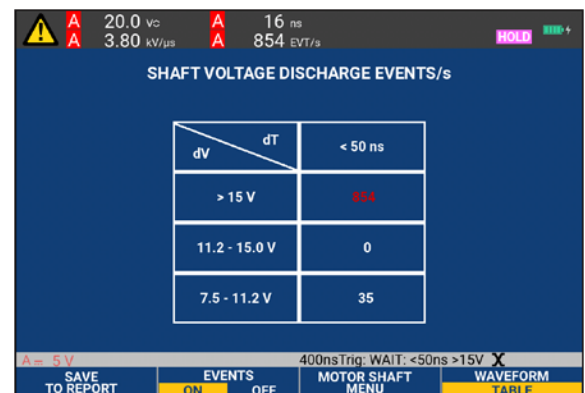
Motor shaft voltage discharge event counts
