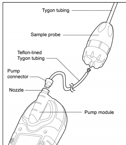
Figure 11. Attaching the Sample Probe
