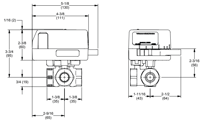
Three-Way Spring Return Two Position Assembly Shipping Weight: 3.0 lbs (1360 g)
