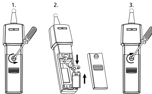
Figure 12: Replacing battery
