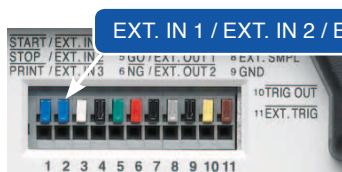
Control terminals
