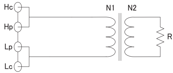
Measuring circuit for turn ratio of windings
