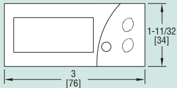
Panel Cutout 2-51/64" x 1-9/64" (71 x 29 mm)
