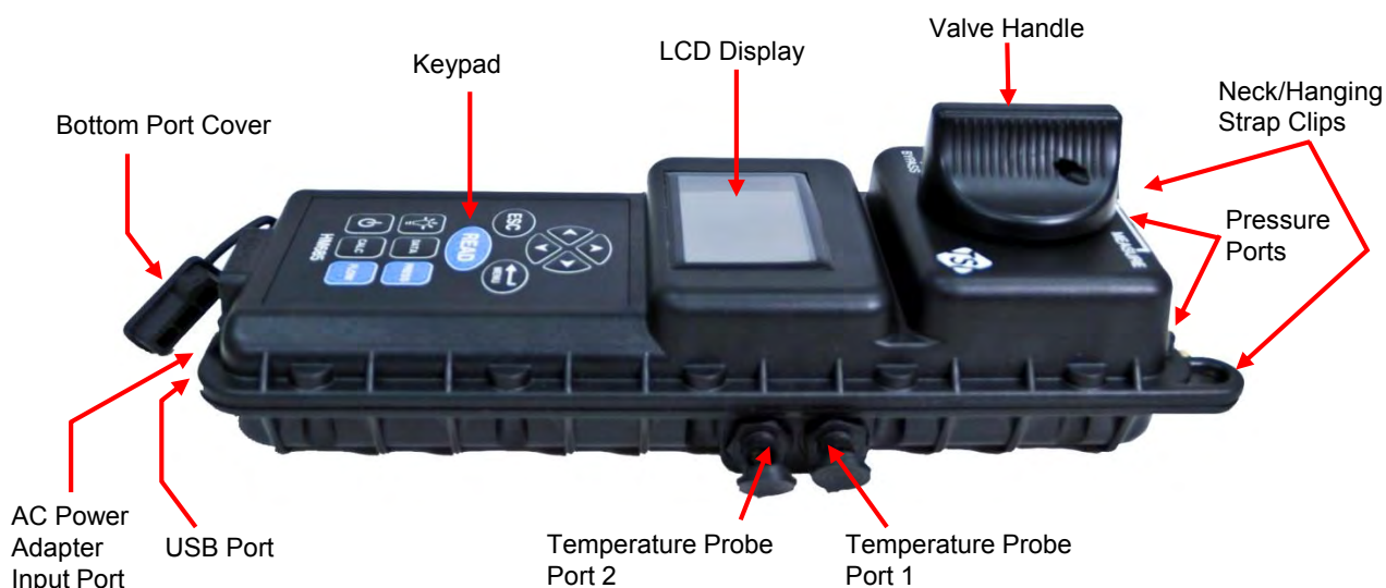
Figure 1-1 HM685 Meter Description
