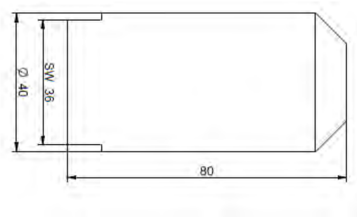
Figure 8: Dimensions (in mm) of the LDP MC measurement chamber base body.
