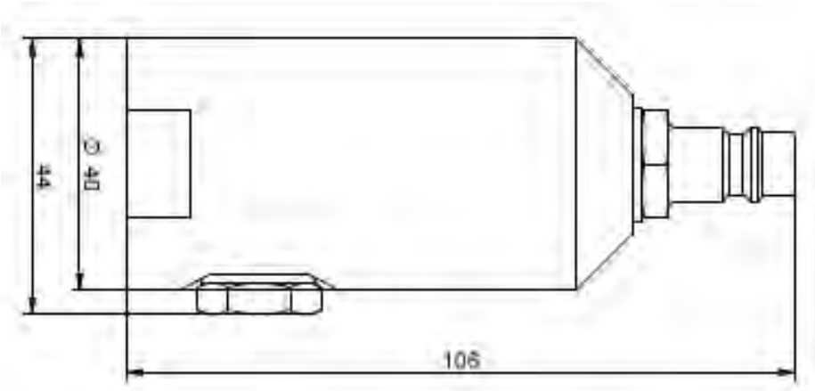
Figure 7: Dimensions (in mm) of the complete measurement chamber with LDP FC fixed valve.
